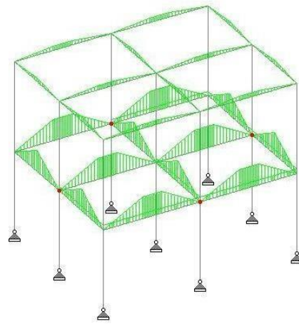
Fig. 7. Dead Load Simulation.
